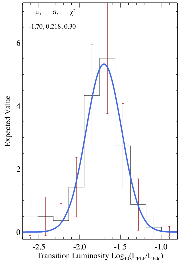
Figure 9. A fit to the distribution of state transition luminosity of PL during index transition after accounting for the x -axis errors using the Monte Carlo simulations described in the text. The mean value of the log ELF, its standard deviation, and the reduced \chi^2 are given in the upper left. The linear value of the best-fitting model is: 1.99 \pm 1.00 ELF.
