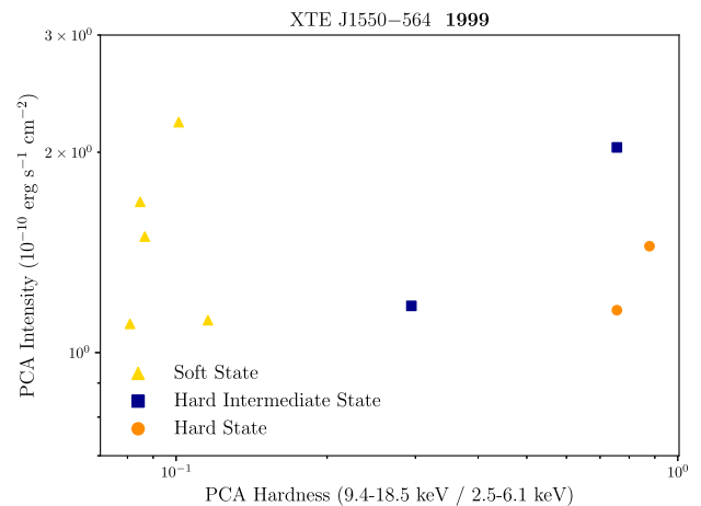
Figure A2. Hardness intensity diagram of XTE J1550–564 in 1999 outburst decay.
