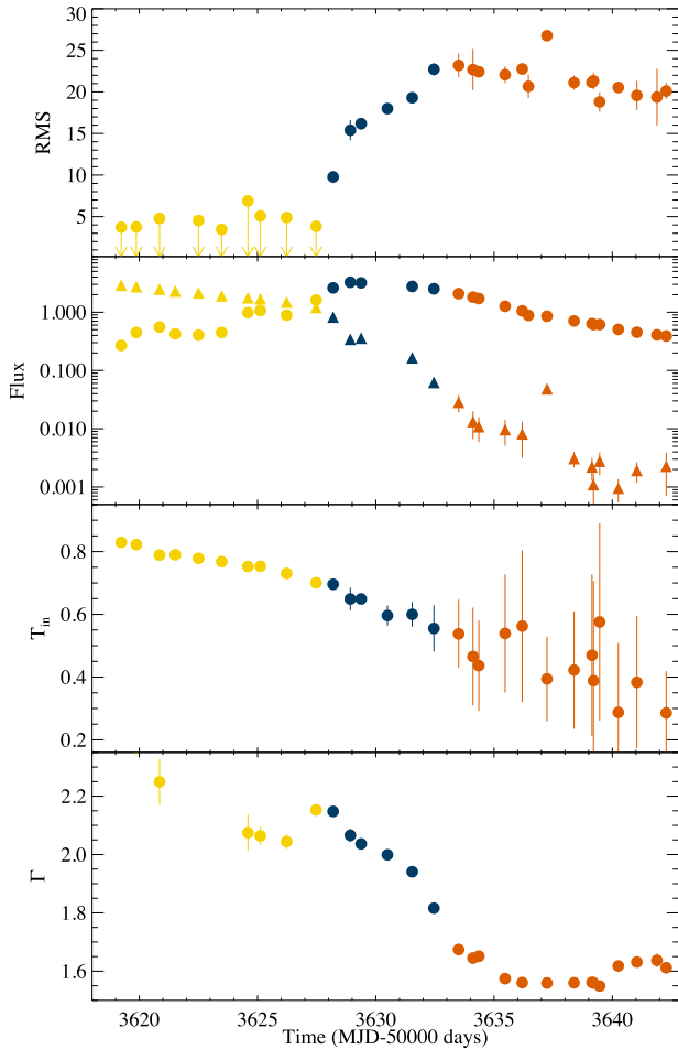
Figure 5. The X-ray spectral and temporal parameters of GRO J1655–40 in 2005 outburst decay as a function of time. (a) rms variability, (b) DBB (shown with triangles) and power law flux (shown with circles) (in 10^{-9} erg s ^{-1} cm ^{-2} ), (c) inner disc temperature (in keV), and (d) X-ray photon index. In the parameter evolution, different states are coloured according to Belloni classification (Table 3) where soft states are presented with yellow colour whereas the hard intermediate (HIMS) and hard states are displayed with blue and orange colour, respectively.
