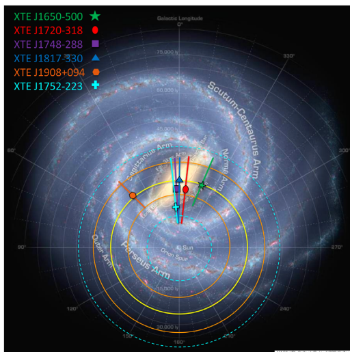
Figure 2. The Galactic distribution of black holes with unknown distance used in this study. The yellow circle displays the 8 kpc radius. Orange circles indicate 1\sigma range used in this work ( 8 \pm 2 kpc) whereas blue dashed lines indicate 2\sigma range. The symbols do not represent the maximum likelihood value, but placed just for presentation purposes. Error bars are arranged from arm to arm or arm towards the Galactic bulge. (Milky Way image: NASA/JPL-Caltech, ESO, J. Hurt.).
