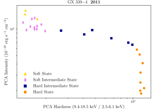
Figure A7. Hardness intensity diagram of GX 339–4 in 2011 outburst decay.
