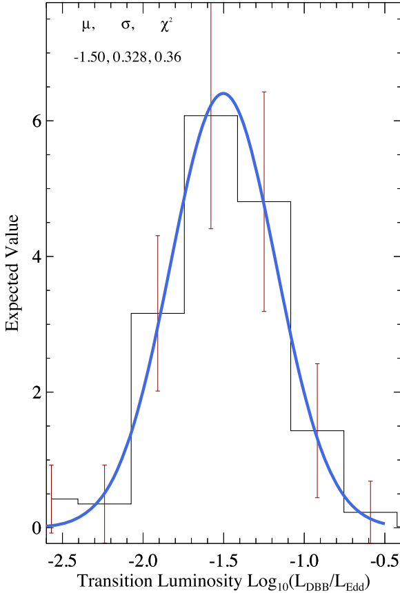
Figure 10. A fit to the distribution of state transition luminosity of DBB during transition to tHIMS after accounting for the x -axis errors using the Monte Carlo simulations described in the text. The mean value of the log ELF, its standard deviation, and the reduced \chi^2 are given in the upper left. The linear value of the best-fitting model is: 3.16 \pm 2.38 ELF.
