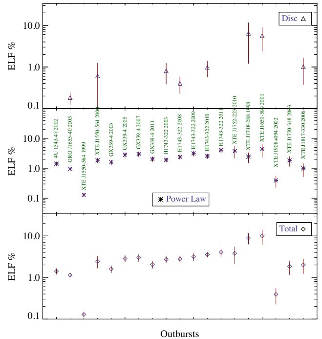
Figure 7. ELF distribution of GBHTs during transition to the hard state. Top: DBB, middle: PL, bottom: total.
