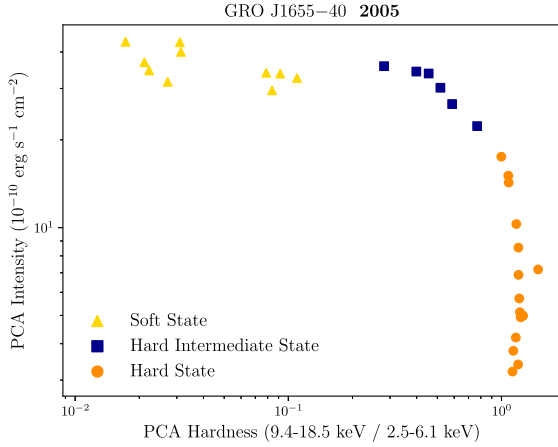
Figure 3. Hardness intensity diagram of GRO J1655–40 in 2005 outburst decay. Different states are coloured according to Belloni classification (Table 3) where soft states are presented with yellow triangle whereas the hard intermediate (HIMS) and hard states are displayed with blue square and orange circle, respectively.
