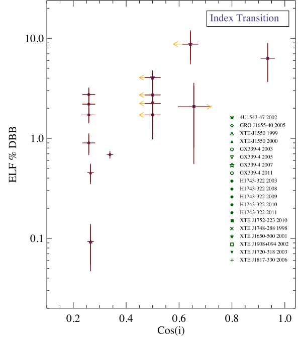
Figure 11. ELF of DBB luminosity as a function of cosine of the inclination angle during index transition. The corresponding references are given in Table 1.
