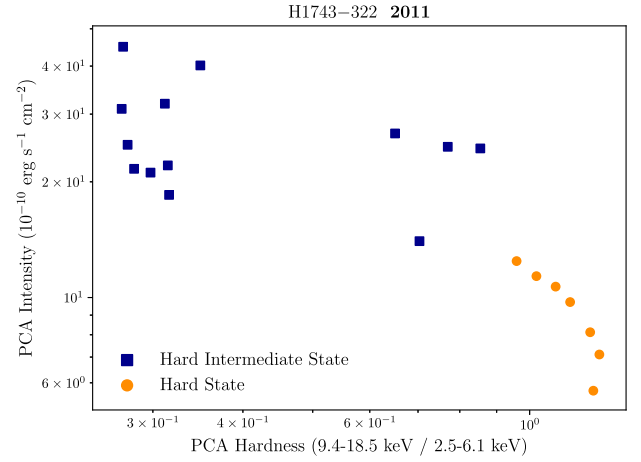
Figure A12. Hardness intensity diagram of H1743-322 in 2011 outburst decay.
