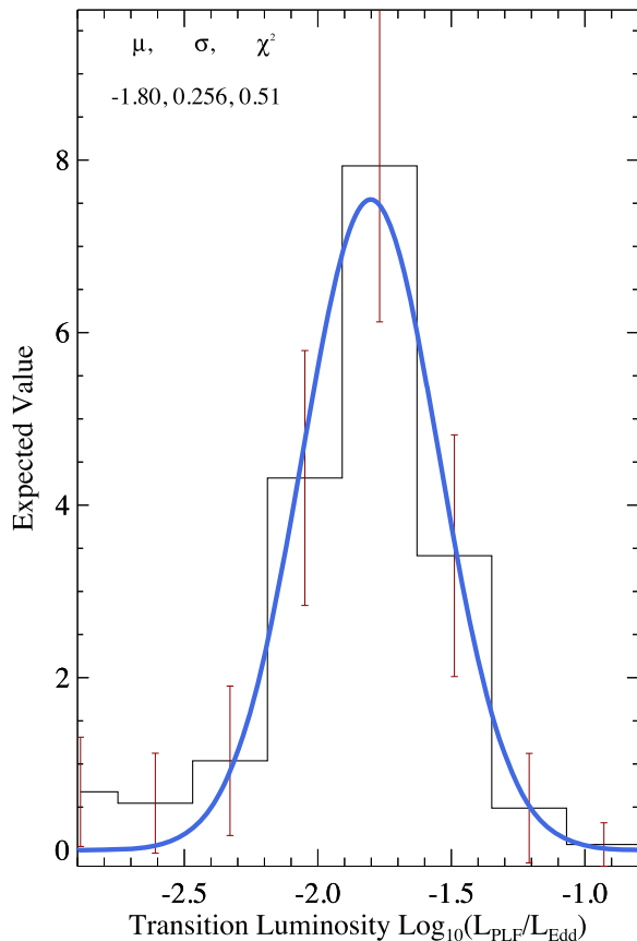
Figure 8. A fit to the distribution of state transition luminosity of PL during transition to the hard state after accounting for the x -axis errors using the Monte Carlo simulations described in the text. The mean value of the log ELF, its standard deviation, and the reduced \chi^2 are given in the upper left. The linear value of the best-fitting model is: 1.58 \pm 0.93 ELF.
