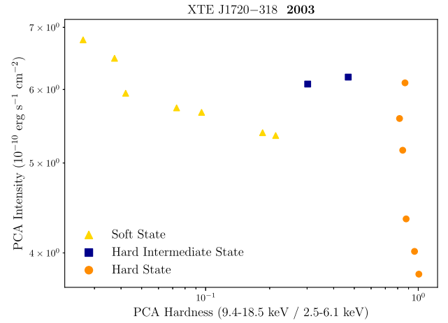
Figure A14. Hardness intensity diagram of XTE J1720-318 in 2003 outburst decay.
