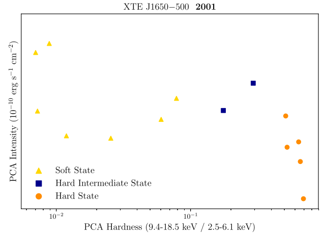
Figure A13. Hardness intensity diagram of XTE J1650-500 in 2001 outburst decay.
