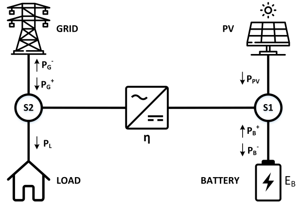
Fig. 1: Nanogrid structure
